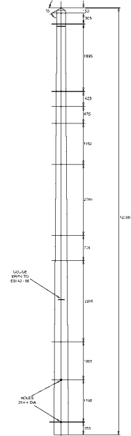
12 METRE POLE FABRICATION
