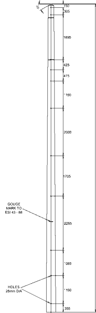
13 METRE POLE FABRICATION
