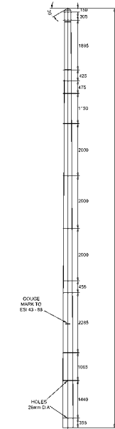
16 METRE POLE FABRICATION
