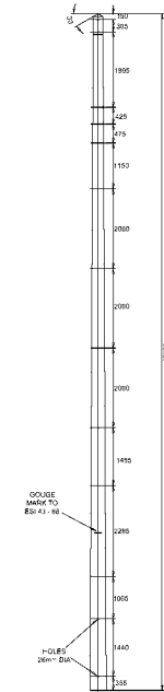
17 METRE POLE FABRICATION
