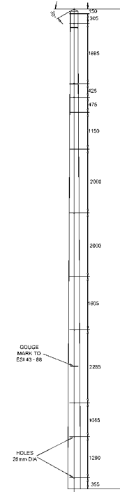
15 METRE POLE FABRICATION
