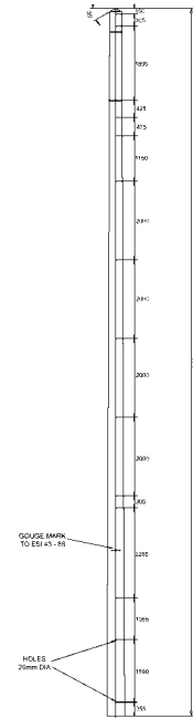
18 METRE POLE FABRICATION
