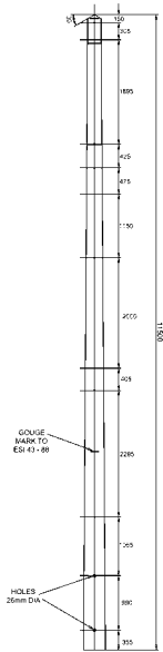
11.5 METRE POLE FABRICATION
